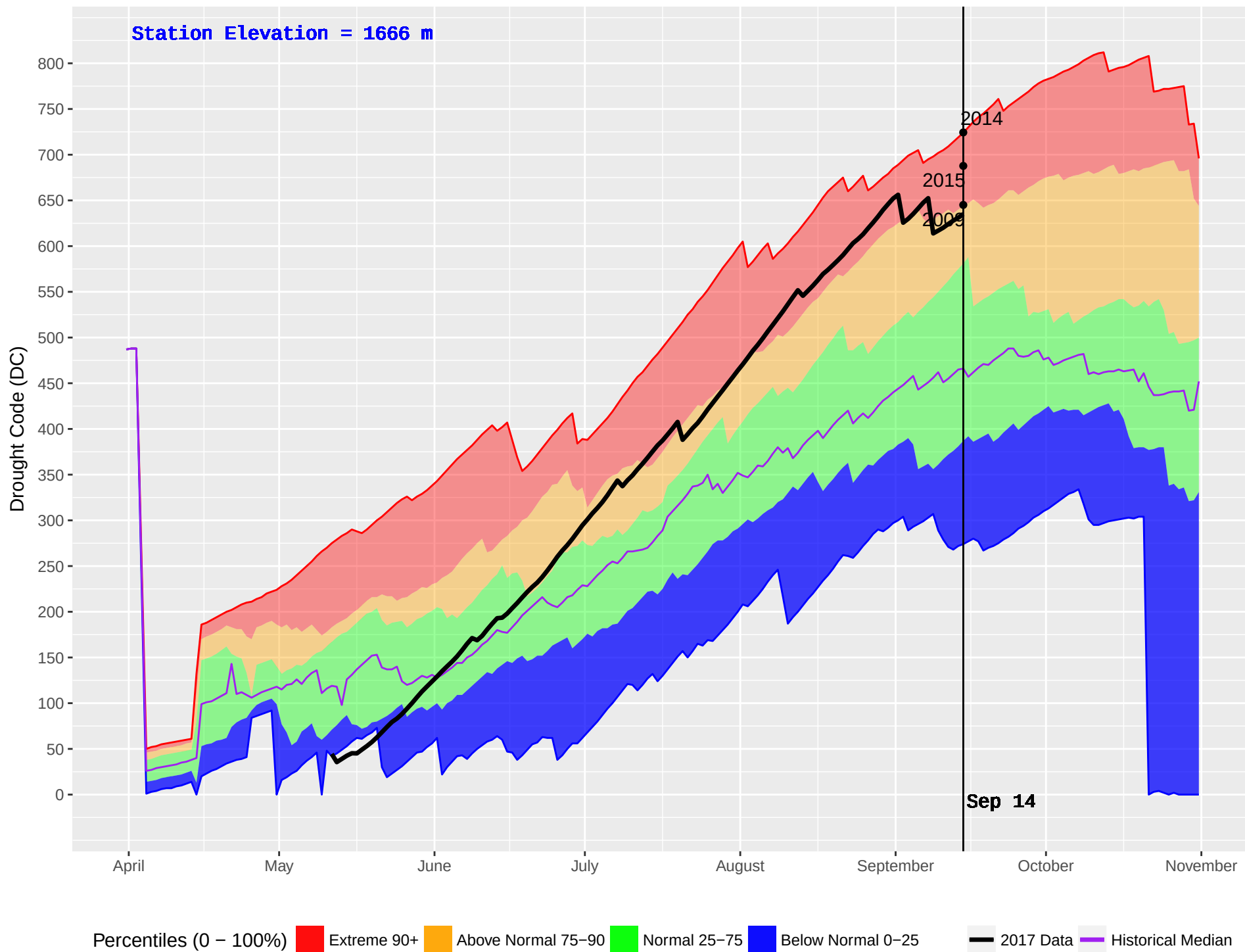
BALDFACE (221) : Historical (1992–2016) and Current (2017) Noon Drought Code (DC)
