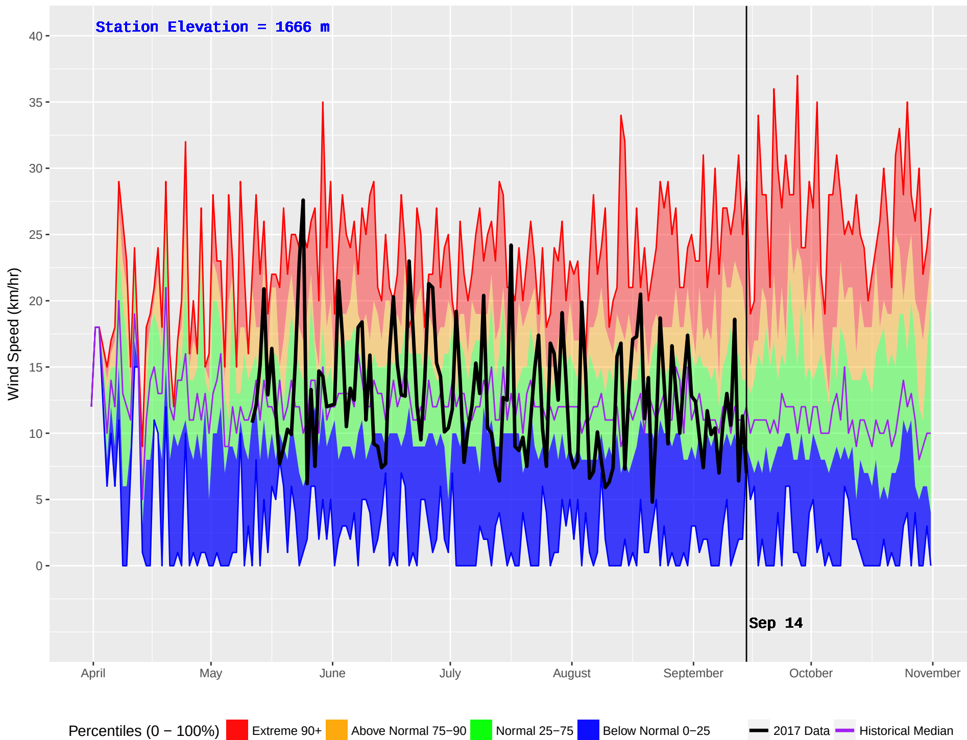
BALDFACE (221) : Historical (1992–2016) and Current (2017) Noon Wind Speed
